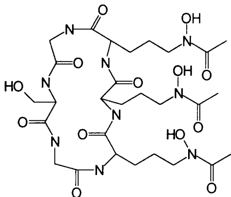
Figure 1. The structure of deferriferrirocrocic acid.
