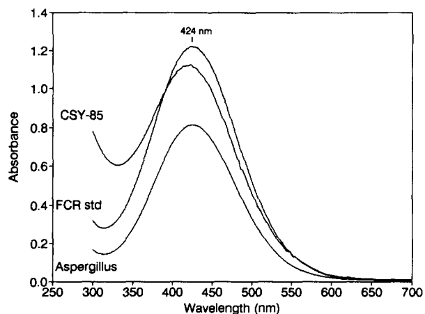
Figure 3. The visible absorbance trace of ferricrocin isolated from W. rehmsii CSY-85, A. fumigatus and ferricrocin obtained as a gift from Professor G. Winkelmann.
